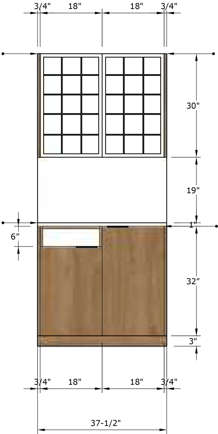
2 Front Elevation
