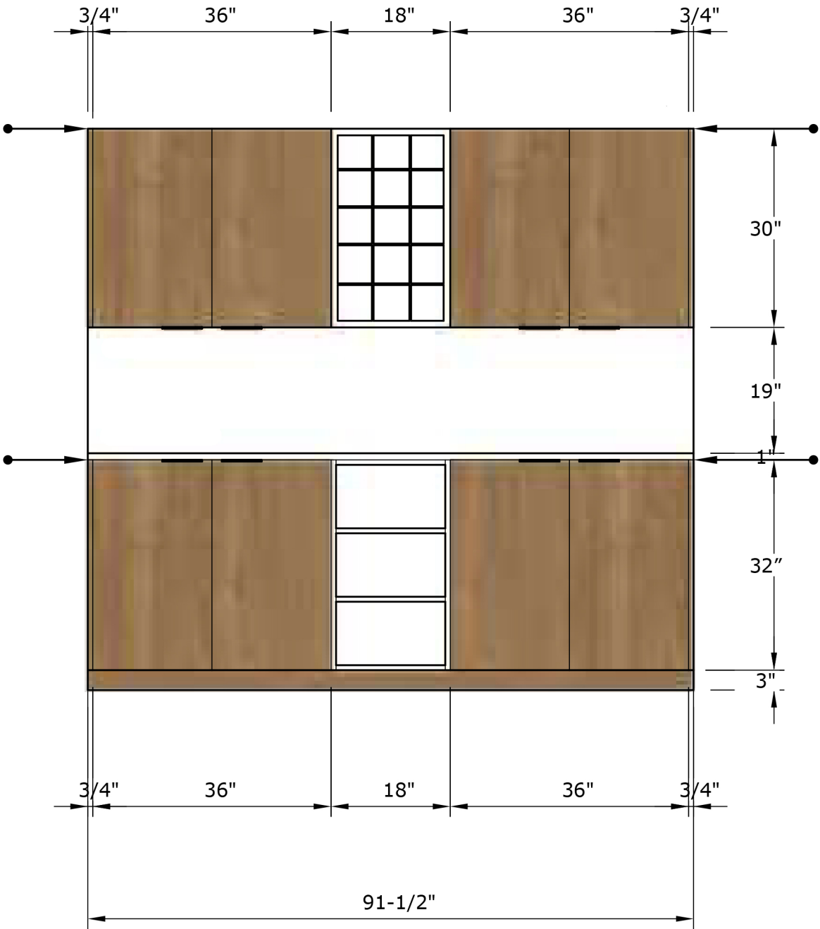
2 Front Elevation
