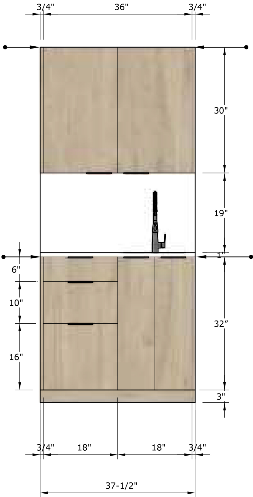
2 Front Elevation
