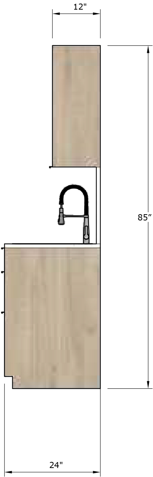
3 Side View
